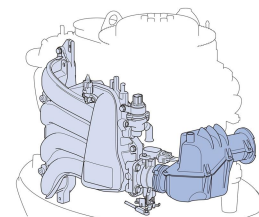
13_F90CF100F_Throttle body, intake manifold and intake blower
